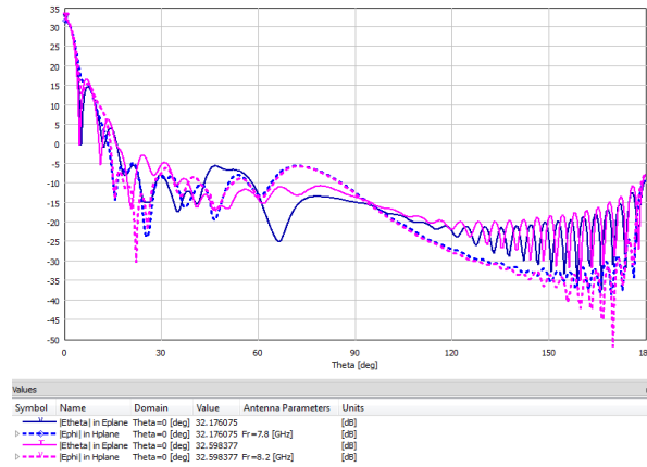
Figure 5: Simulated radiation patterns of the antenna of Fig. 3: in E-plane (continuous) and H-plane (dotted) for the frequencies 7.8 (blue) and 8.2 (magenta) GHz.
