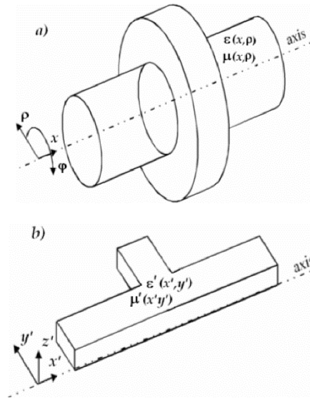
Figure 1: Equivalence between planar and BOR circuits. A planar equivalent of the BOR circuit is filled with inhomogeneous anisotropic materials.
