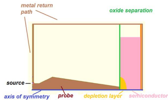
Figure 12: QW-V2D model for the tip of the Keysight SMM probe after [15].
