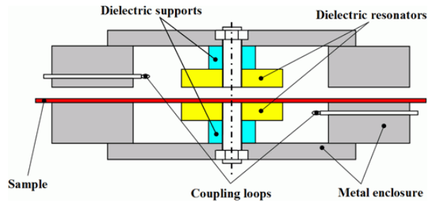
Figure 10: A split - post dielectric resonator (SPDR) [2].
