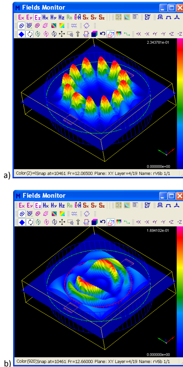
Figure 9: E - field distribution of two modes in a cylindrical dielectric resonator at close resonant frequencies of 12.065 GHz (a) and 12.66 GHz (b).
