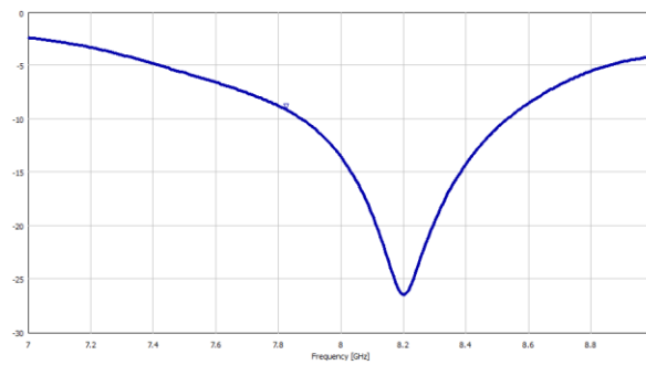
Figure 6: Simulated return loss of the antenna of Fig. 3 ( |S_{11}| versus frequency in 7÷9 GHz band).
