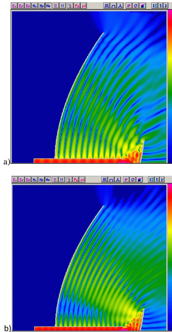
Figure 8: Maximum value of H_\phi field in steady state operation of a dual-reflector antenna in logarithmic scale from maximum (purple) down to -60 dB (blue), at 11.7 GHz (a) and 14.1 GHz (b).
